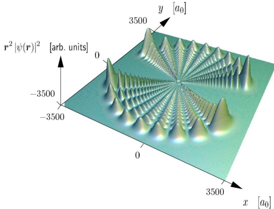
FIG. 1: (color online.) The number of terms in the radial wave function grows with the principal quantum number n and with the angular momentum defect \zeta = n - l . In order to illustrate this well-known fact, we here plot the radial probability density of the state with quantum numbers n = 40 , l = 14 and m = 6 , in the plane of constant azimuth \phi = 0 . Here, a_0 denotes the Bohr radius a_0 = \hbar/(\alpha mc) = 0.529\,177\,2108(18) \times 10^{-10} m [16]. The Bethe logarithm for the state under discussion reads \ln k_0(n=40, l=14) = -0.418\,087\,713 \times 10^{-4} .
