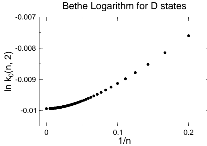
FIG. 2: The Bethe logarithms for l = 2 are in excellent agreement with their asymptotic limit as n \rightarrow \infty . We plot here the values \ln k_0(n, 2) as a function of n^{-1} . For n = 190, \dots, 200 , the values of \ln k_0(n, 2) are given in Table II (see Ref. [52] for a complete list of all relevant values in the range n \leq 200 ). The limiting value at n^{-1} = 0 , which is \ln k_0(\infty, 2) = -0.994\,045\,690 \times 10^{-2} (see also Table V), has been evaluated independently according to Ref. [46].
